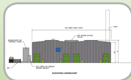
Proposed energy facility elevation looking east
